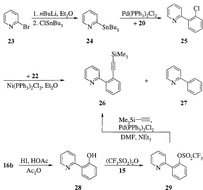
Scheme 5. The preparation of 2-{2-[2-(trimethylsilyl)ethynyl]phenyl}pyridine ( 26 )
