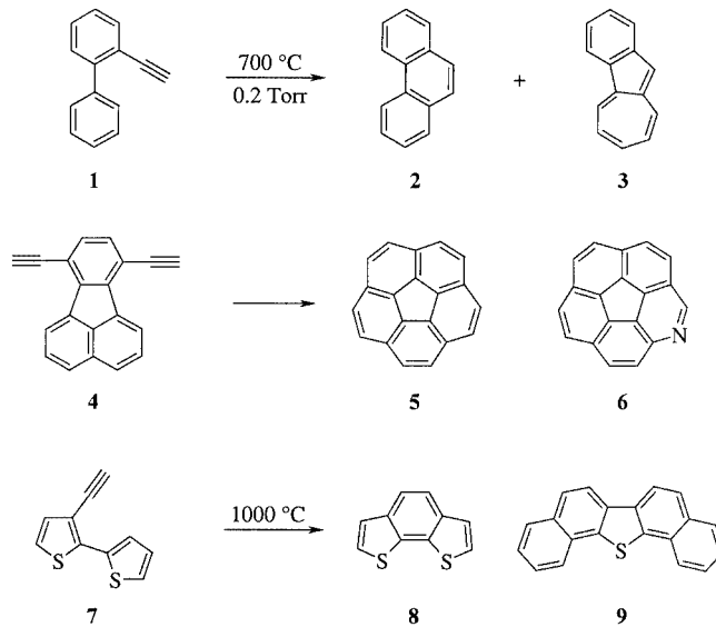
Scheme 1. Condensed aromatics and heteroaromatics by pyrolysis of alkynes
