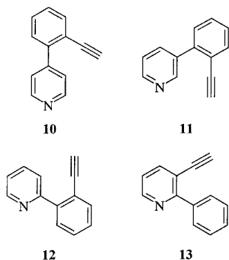
Scheme 2. A selection of (ethynylphenyl)pyridine derivatives
