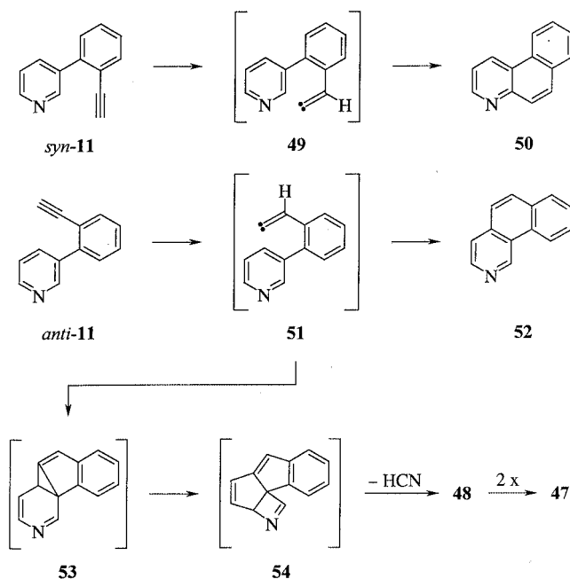
Scheme 9. The pyrolysis of 3-(2-ethynylphenyl)pyridine ( 11 )
