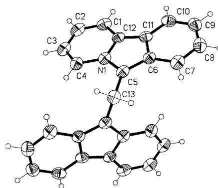
Figure 1. The structure of 37 in the crystal
