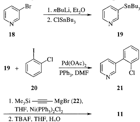
Scheme 4. The preparation of 3-(2-ethynylphenyl)pyridine ( 11 )
