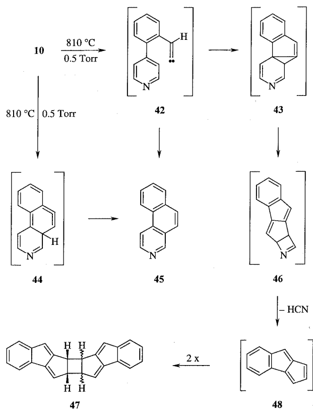
Scheme 8. The pyrolysis of 4-(2-ethynylphenyl)pyridine ( 10 )
