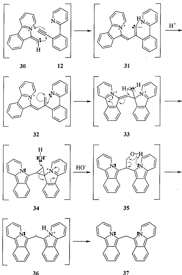
Scheme 6. The "dimerization" of 2-(2-ethynylphenyl)pyridine ( 12 )
