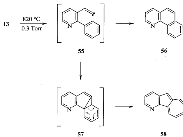
Scheme 10. The pyrolysis of 3-ethynyl-2-phenylpyridine ( 13 )
