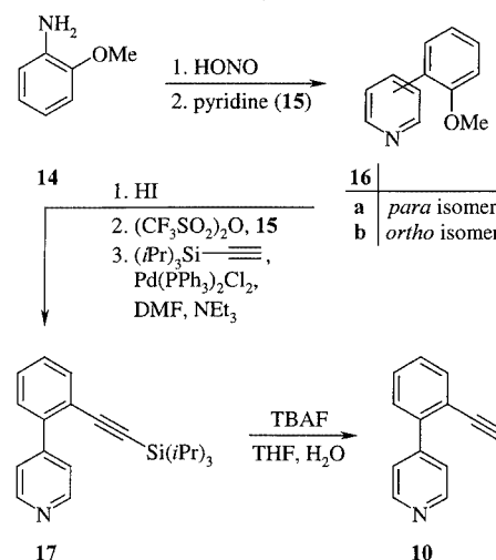
Scheme 3. The preparation of 4-(2-ethynylphenyl)pyridine ( 10 )
