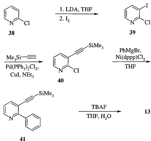
Scheme 7. The preparation of 3-ethynyl-2-phenylpyridine ( 13 )
